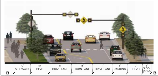
STREET SECTION B-B AT WARD COUNTY COURTHOUSE
