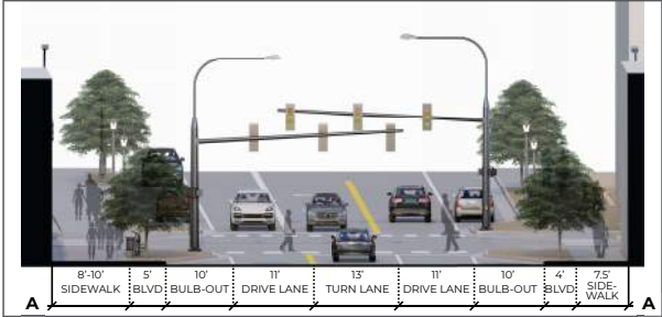
STREET-SECTION A-A BASE ALT 1B OPTION 1-2
