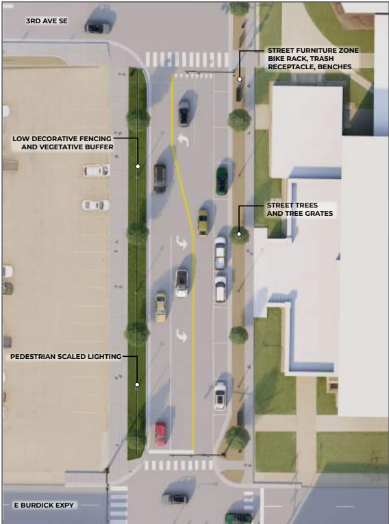
ENLARGED PLAN BASE ALT 1B
