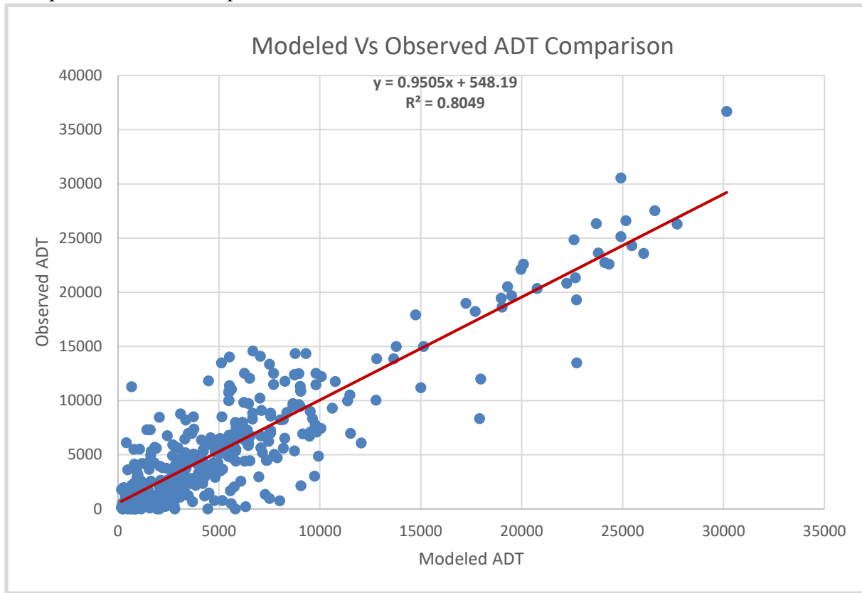
Figure 6 Scatter Plot of Modeled and Observed ADTS
